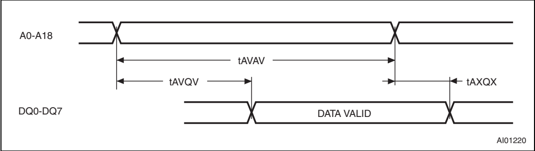
Figure 5. Address controlled, READ mode AC waveforms
