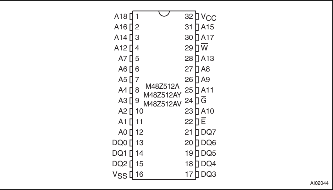
Figure 2. DIP connections
